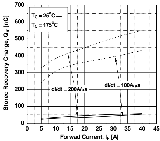
Figure 23. Stored Charge
